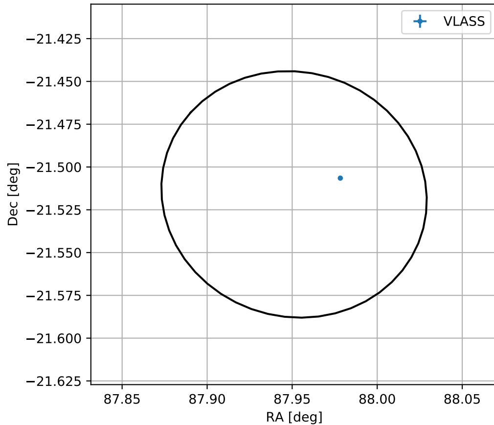
4FGL J0551.8-2130
