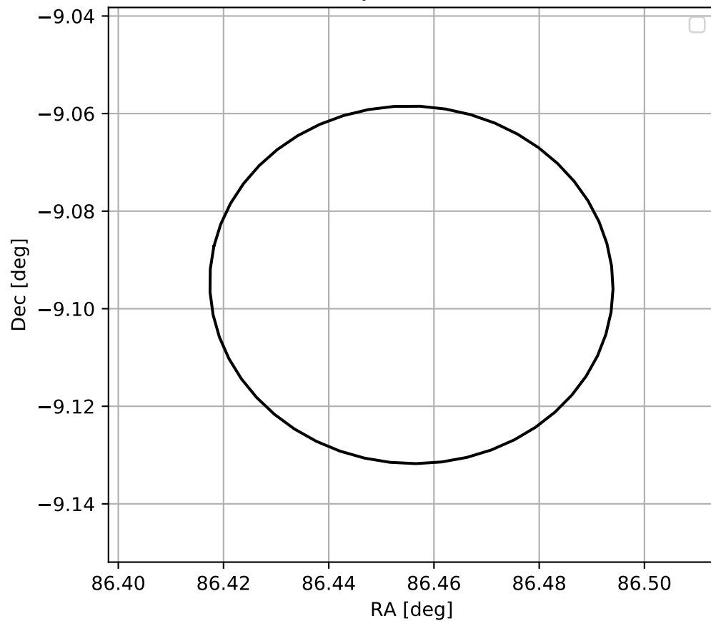
4FGL J0545.8-0905
