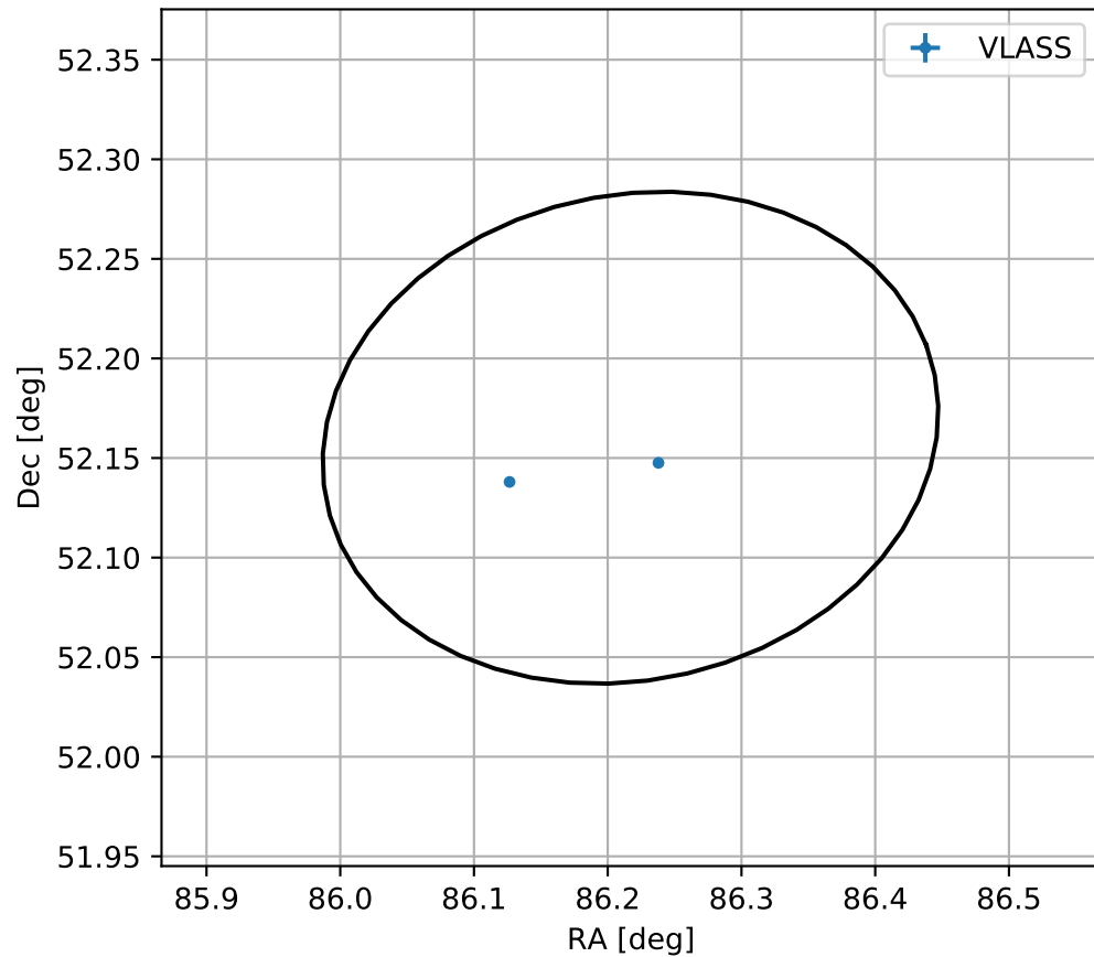
4FGL J0544.8+5209c
