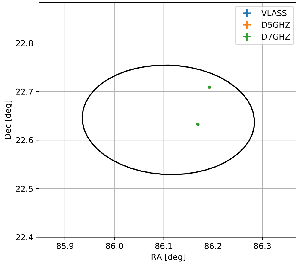
4FGL J0544.4+2238
