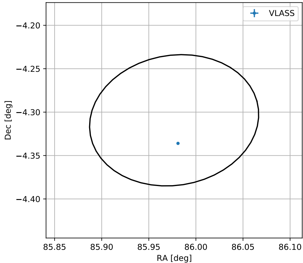
4FGL J0543.9-0418
