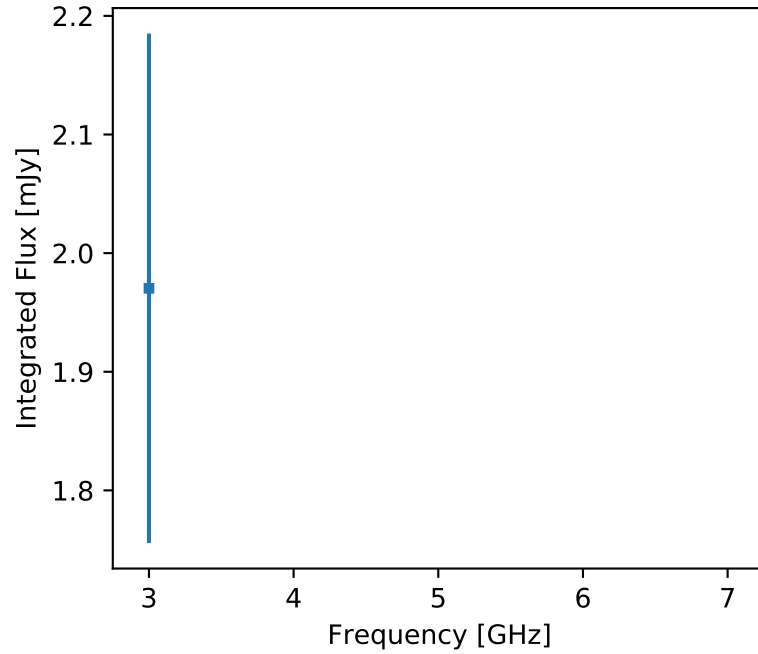
F357 J054105.50+361611.7 (unr)
