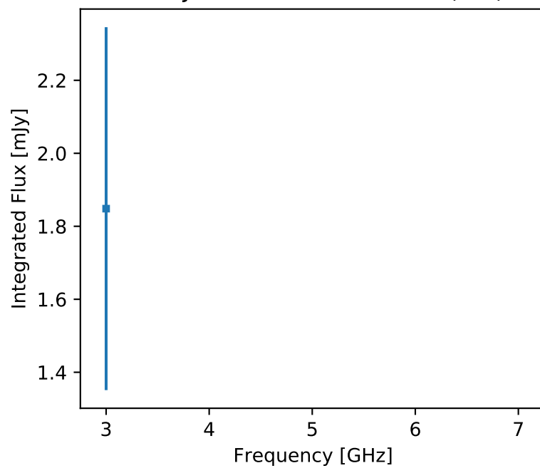
F357 J054052.04+361806.8 (res)
