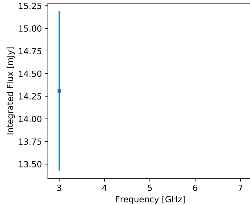
F357 J054105.50+361611.7 (unr)
