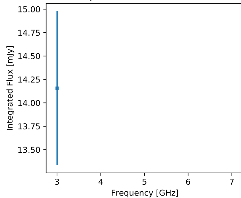
F357 J054052.04+361806.8 (res)
