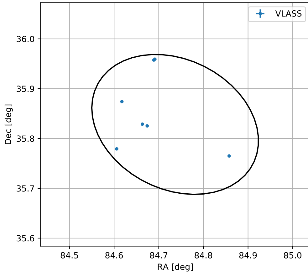
4FGL J0538.9+3549c
