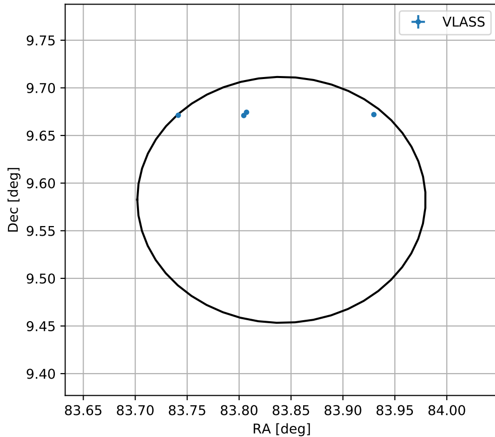
4FGL J0535.3+0934
