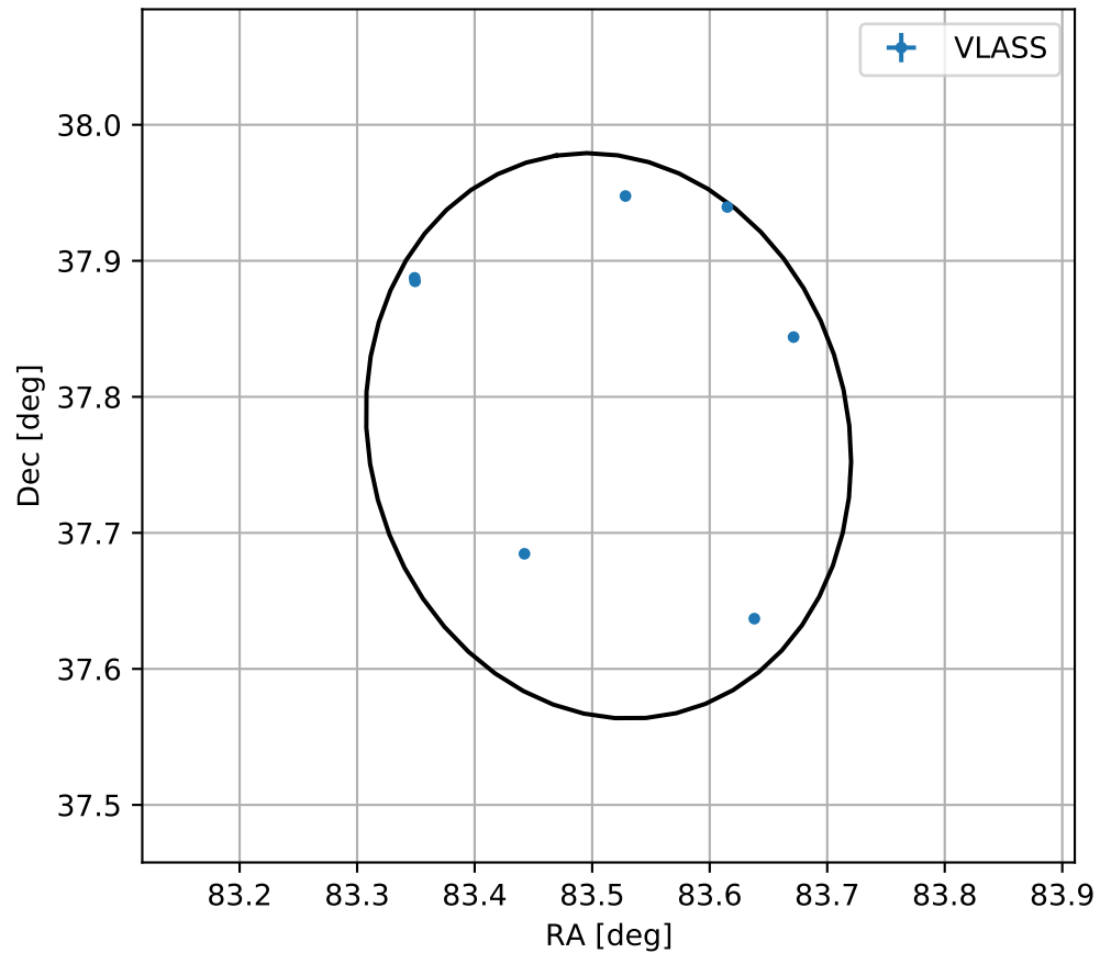
4FGL J0534.0+3746c
