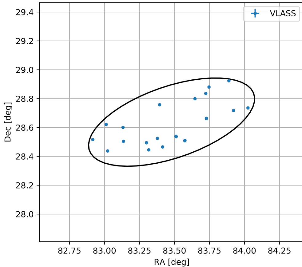
4FGL J0533.9+2838
