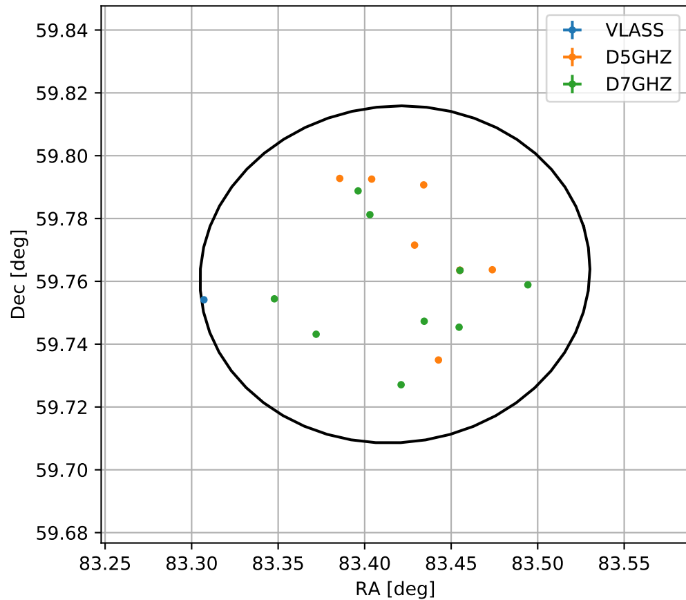
4FGL J0533.6+5945
