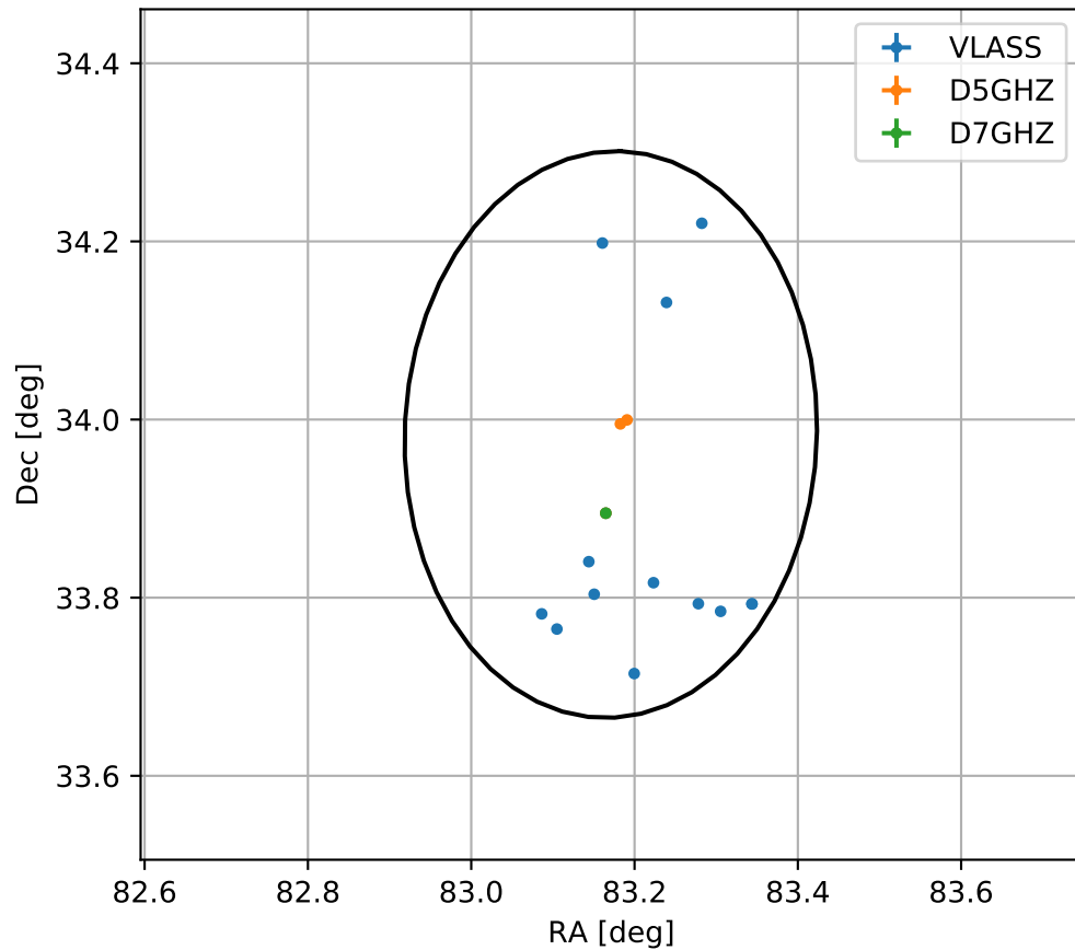
4FGL J0532.6+3358
