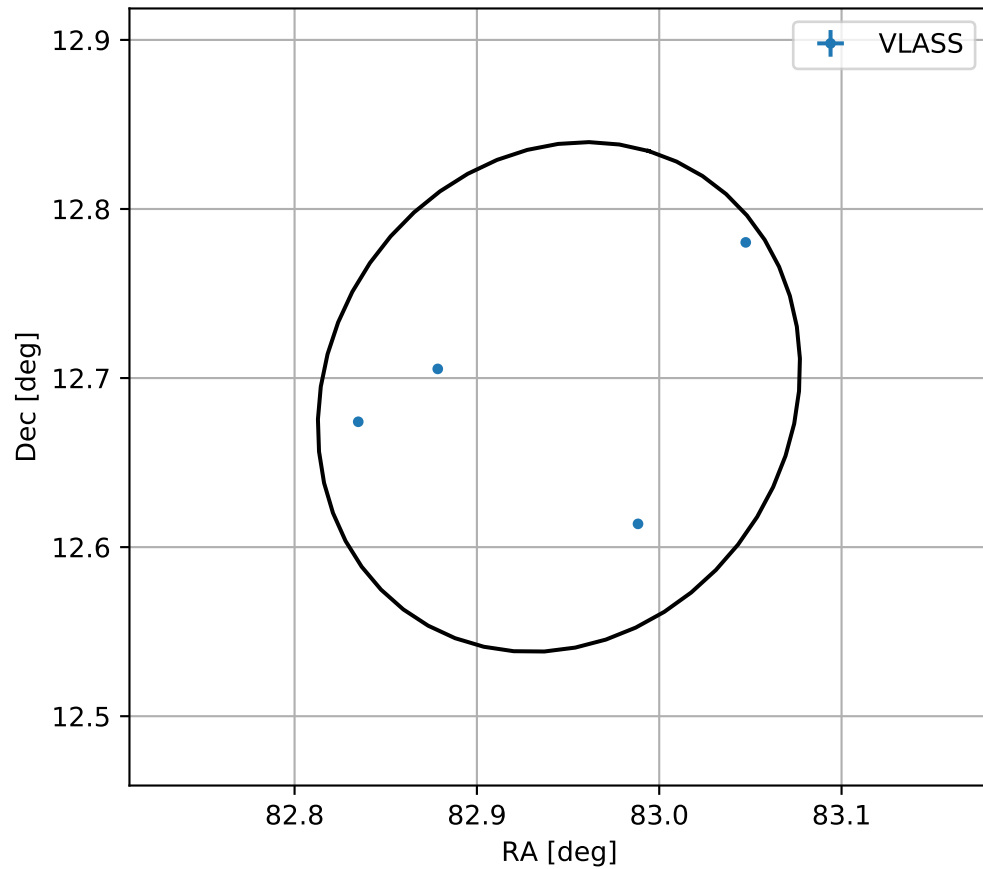
4FGL J0531.7+1241c
