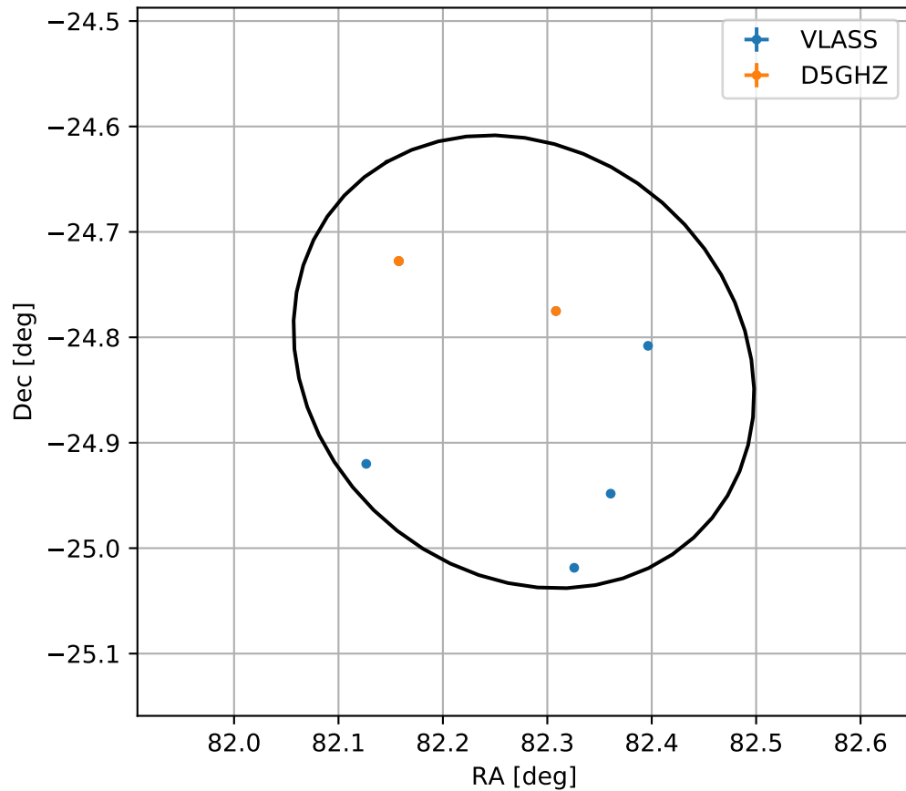
4FGL J0529.1-2449c
