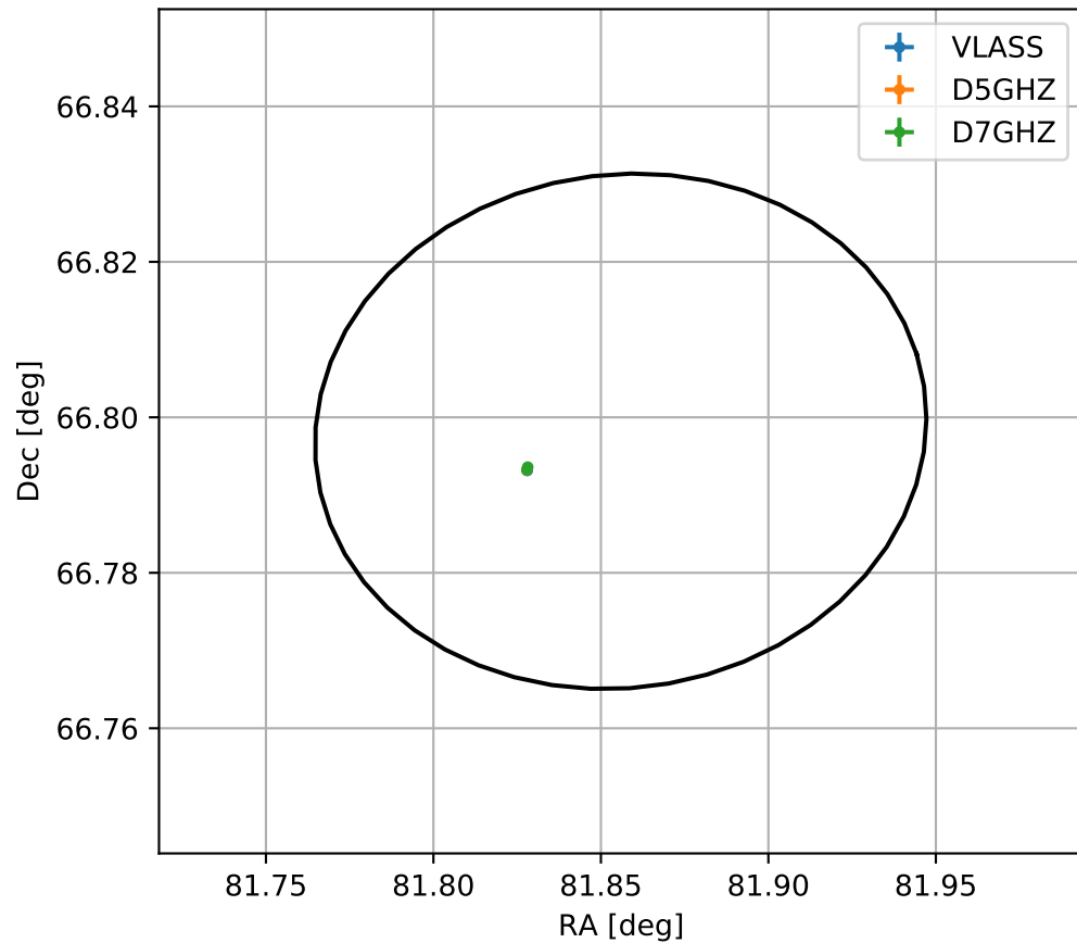
4FGL J0527.4+6647
