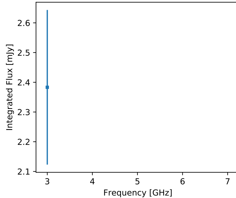
F357 J052731.01+115113.4 (unr)
