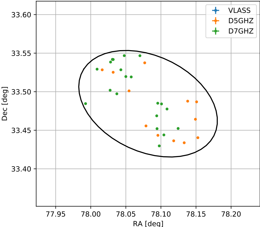
4FGL J0512.3+3329
