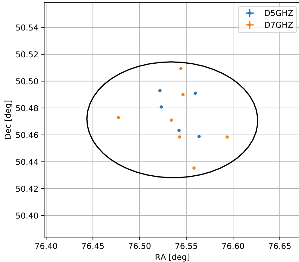
4FGL J0506.1+5028
