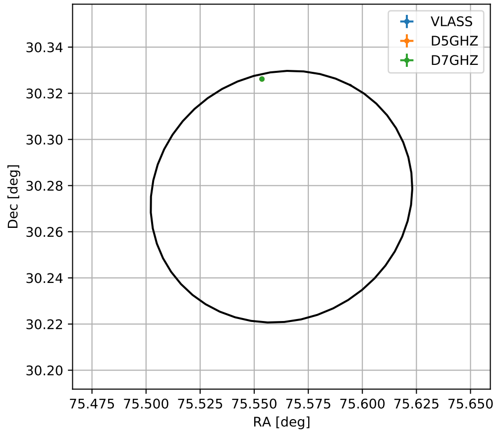
4FGL J0502.2+3016
