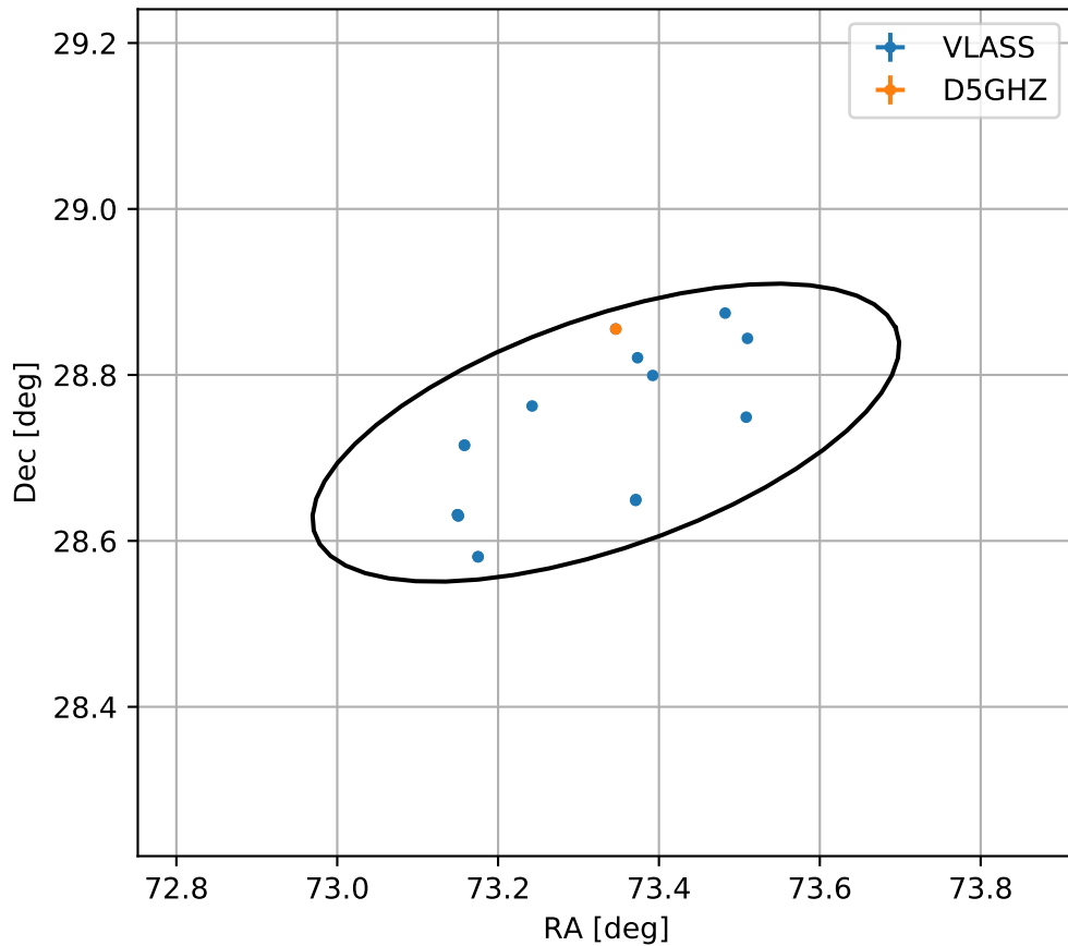
4FGL J0453.3+2843
