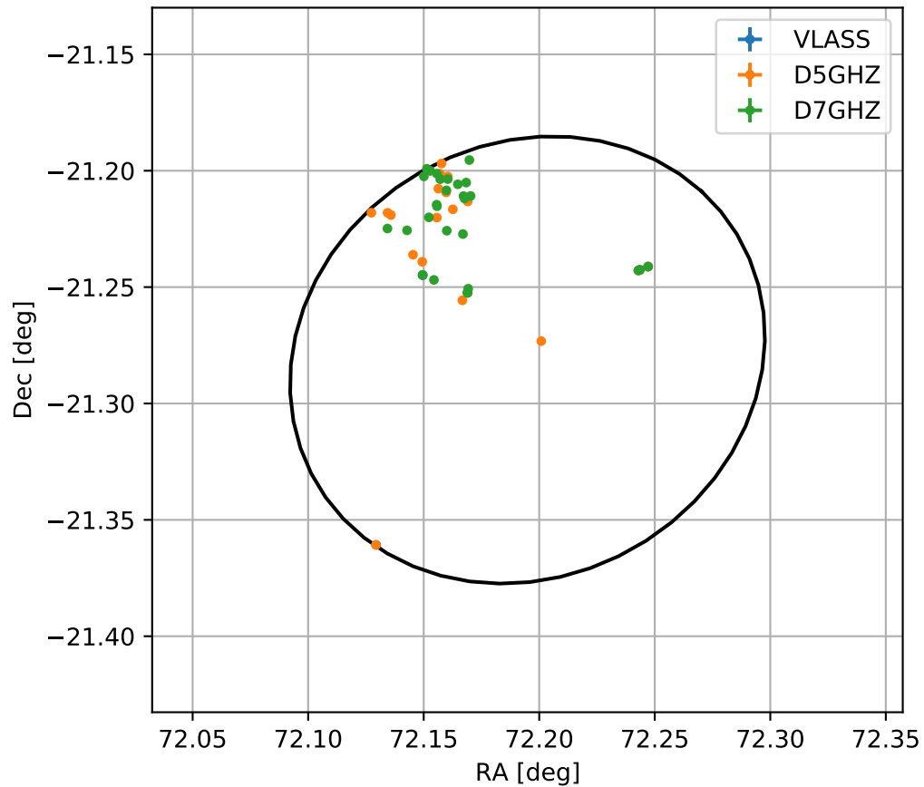
4FGL J0448.7-2116
