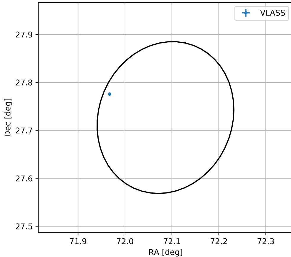
4FGL J0448.3+2743
