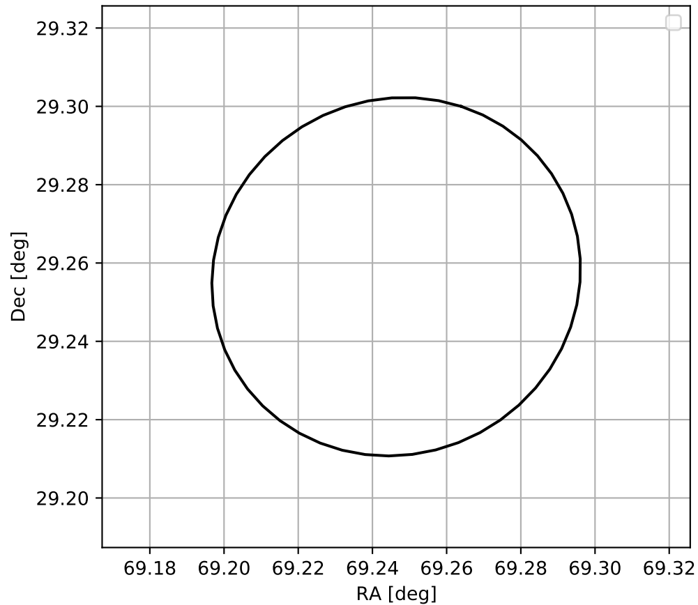
4FGL J0436.9+2915
