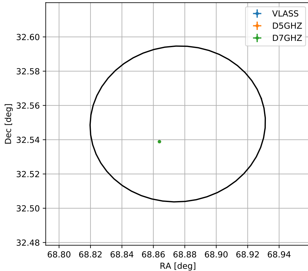
4FGL J0435.5+3232
