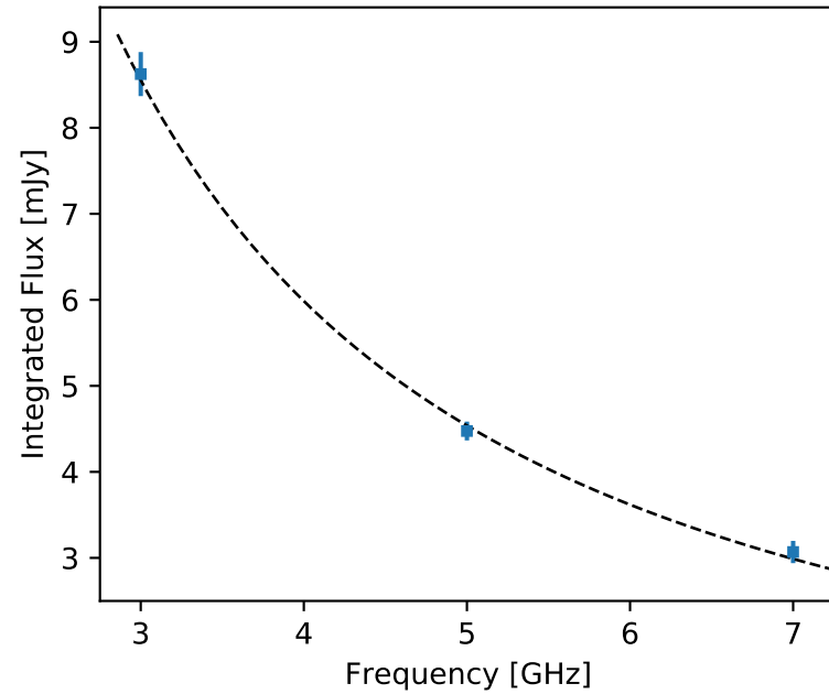
F357 J043527.32+323219.8 (unr)
