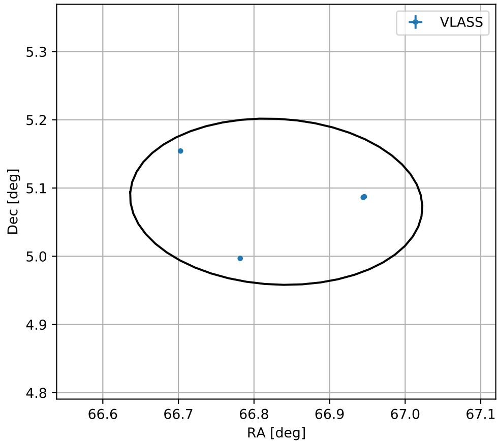
4FGL J0427.3+0504
