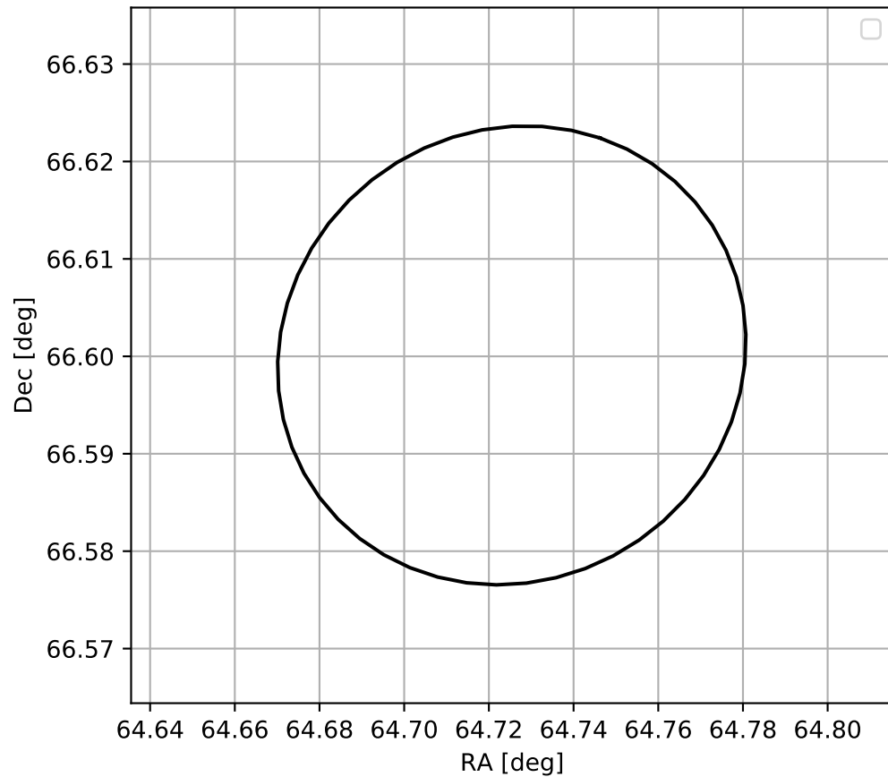
4FGL J0418.9+6636
