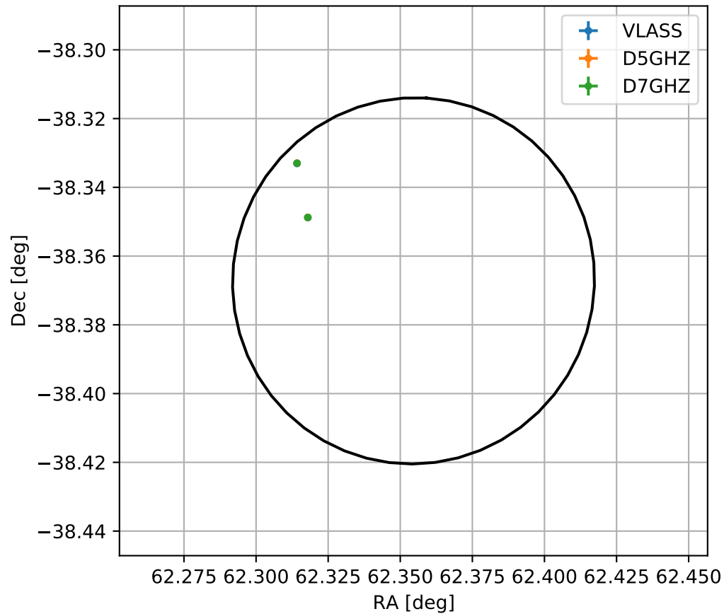
4FGL J0409.4-3822
