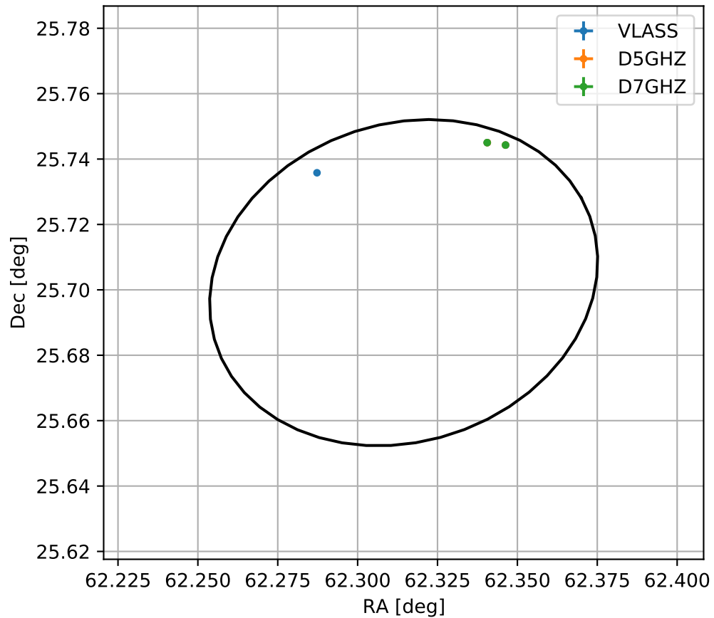
4FGL J0409.2+2542
