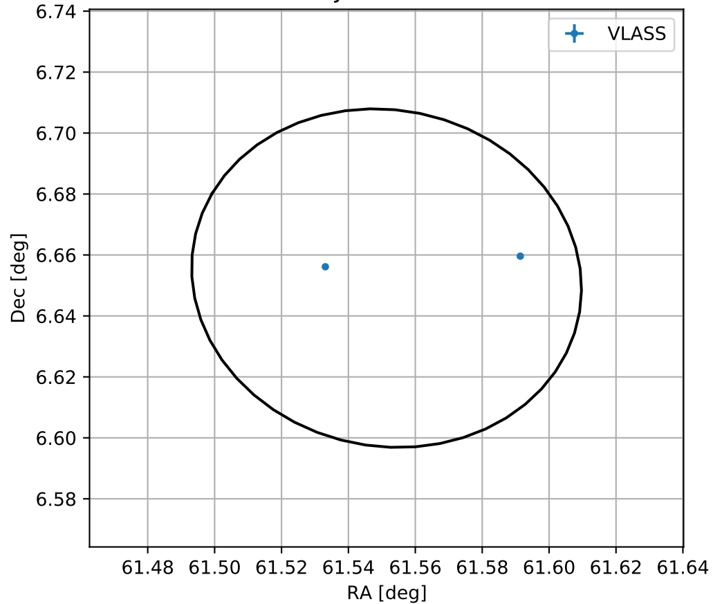
4FGL J0406.2+0639
