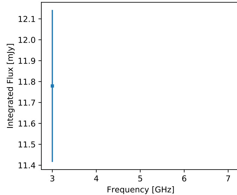
F357 J040621.93+063934.5 (unr)
