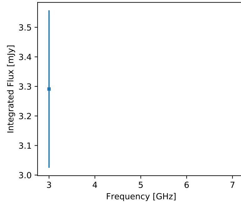
F357 J040328.64+125052.0 (unr)
