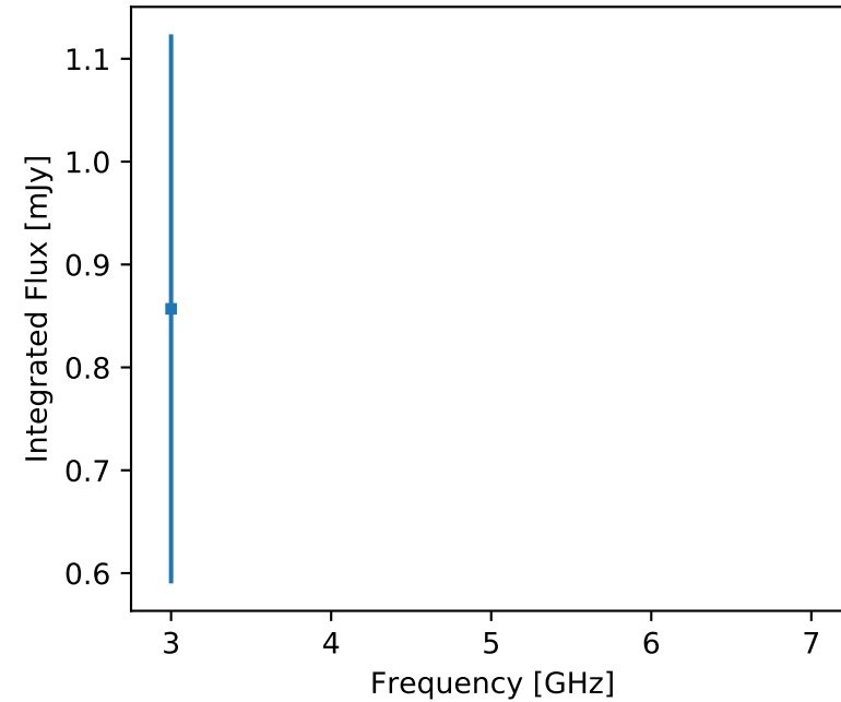
F357 J040328.64+125052.0 (unr)
