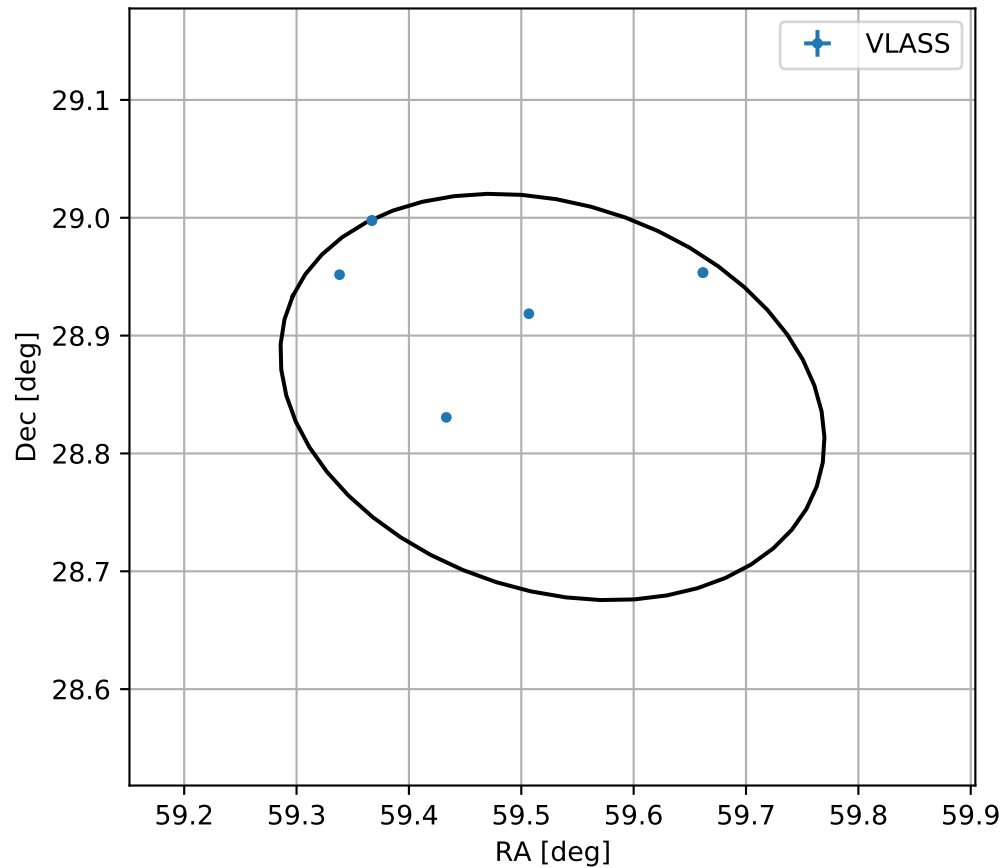
4FGL J0358.1+2850
