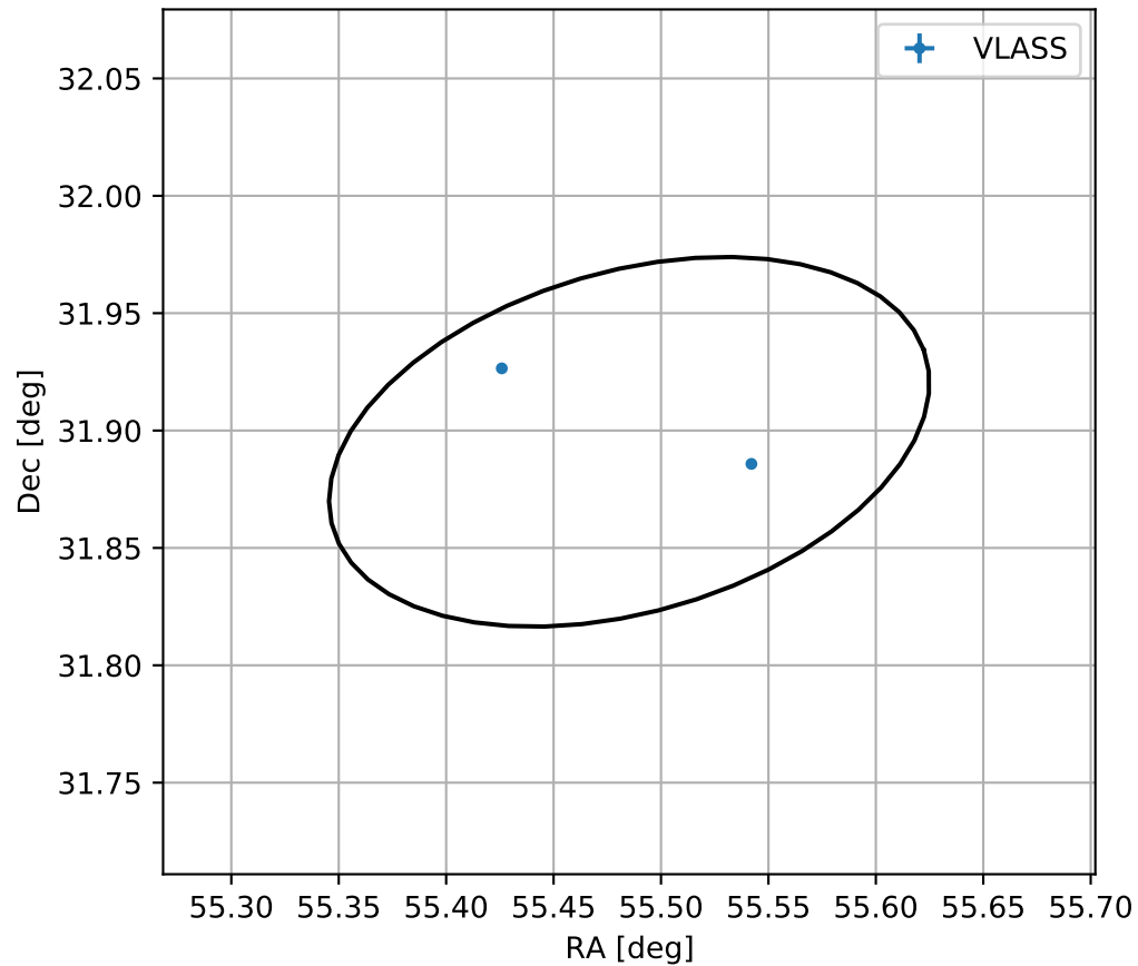
4FGL J0341.9+3153c
