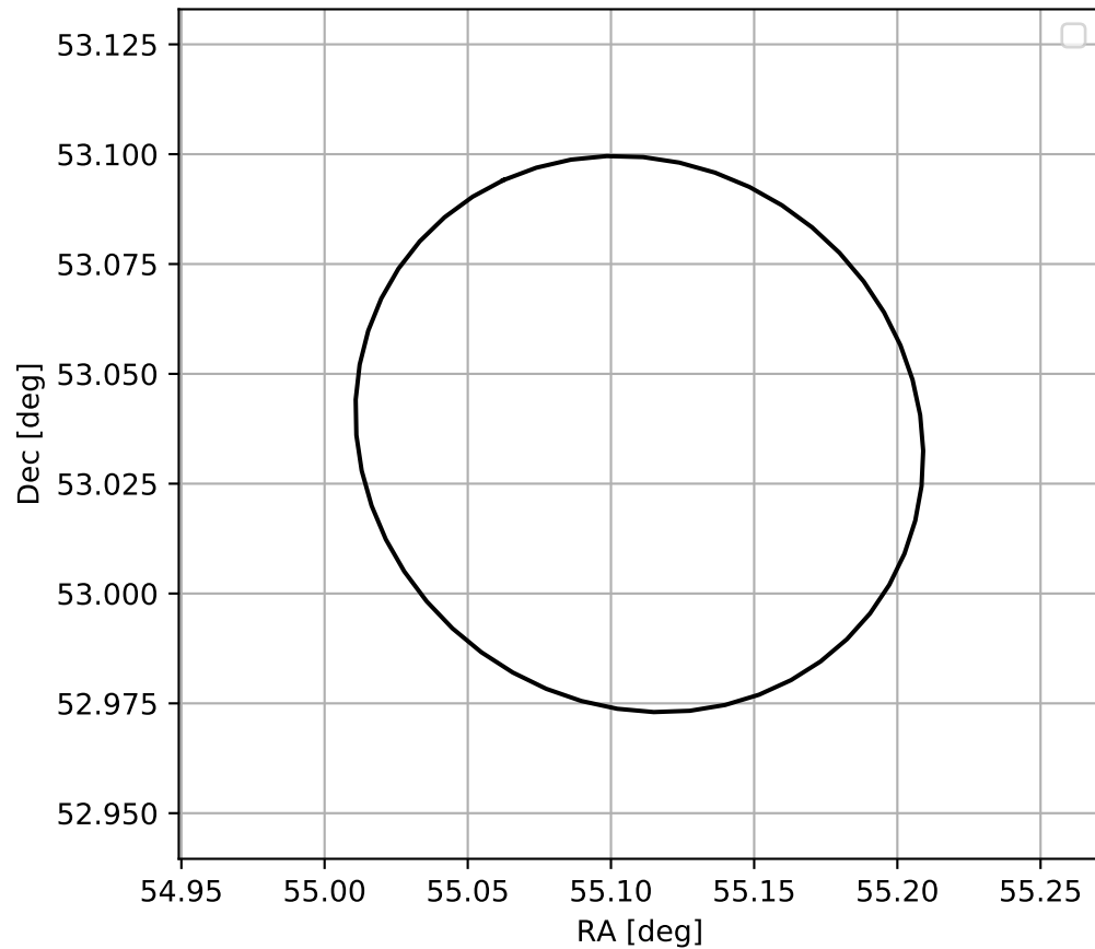
4FGL J0340.4+5302
