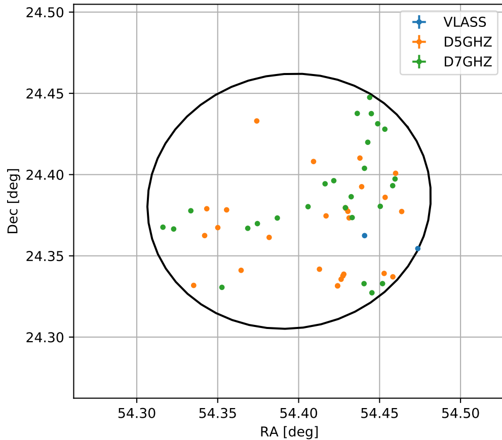
4FGL J0337.5+2423c
