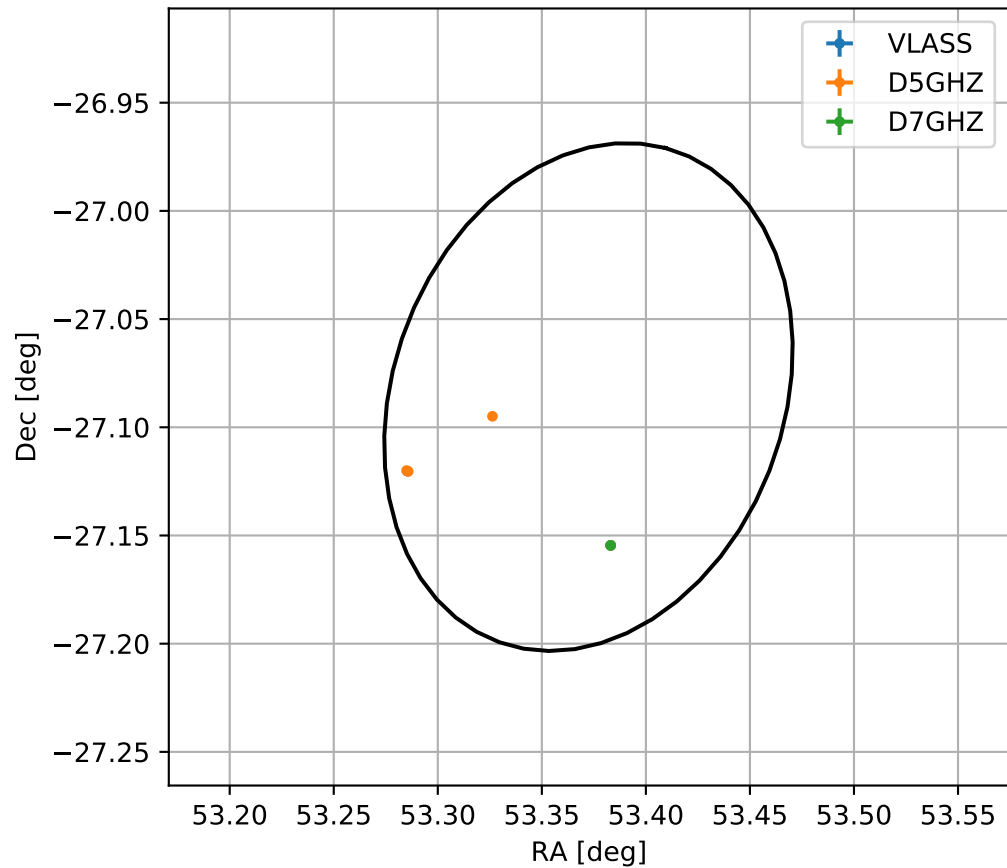
4FGL J0333.4-2705
