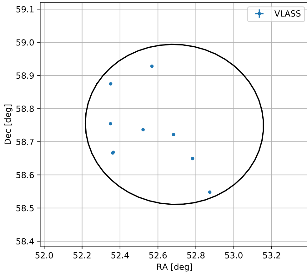
4FGL J0330.7+5845
