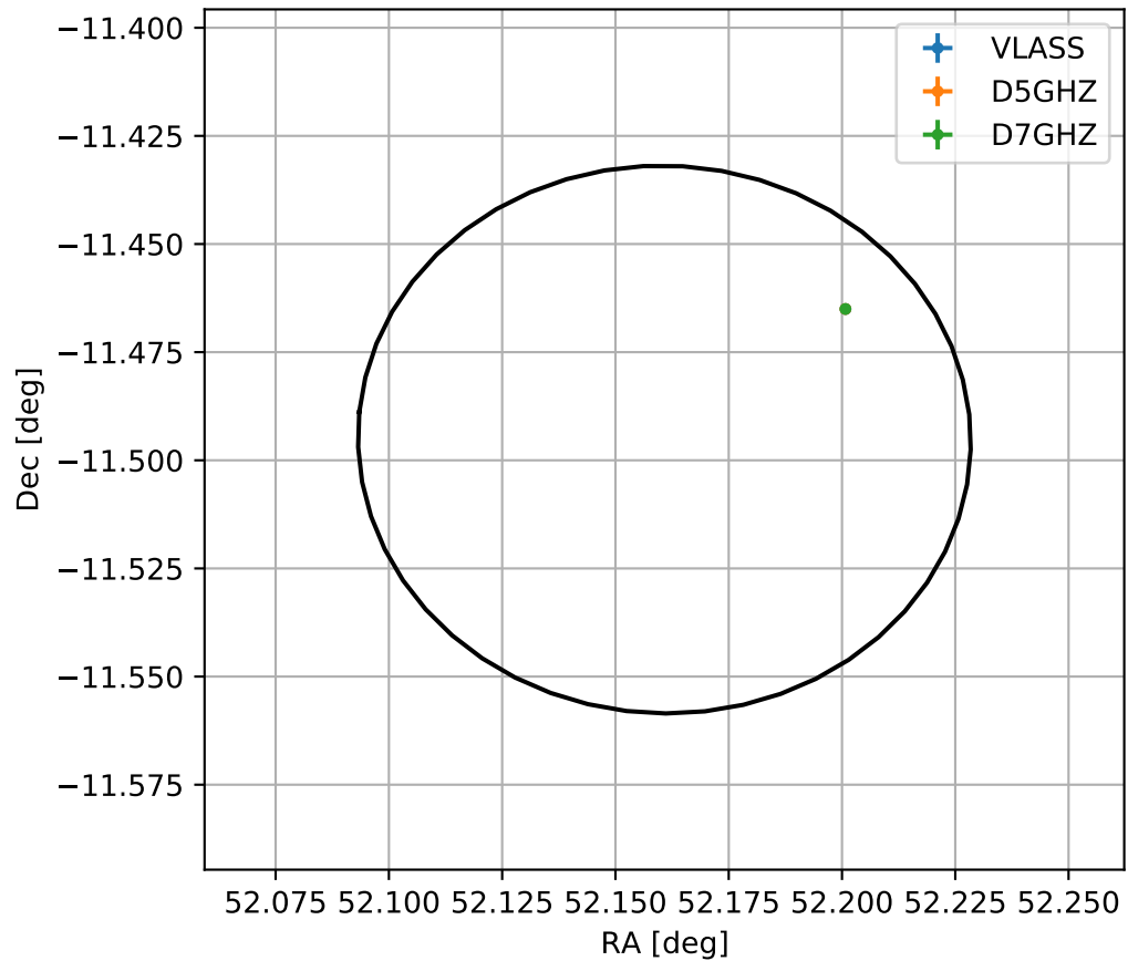
4FGL J0328.6-1129
