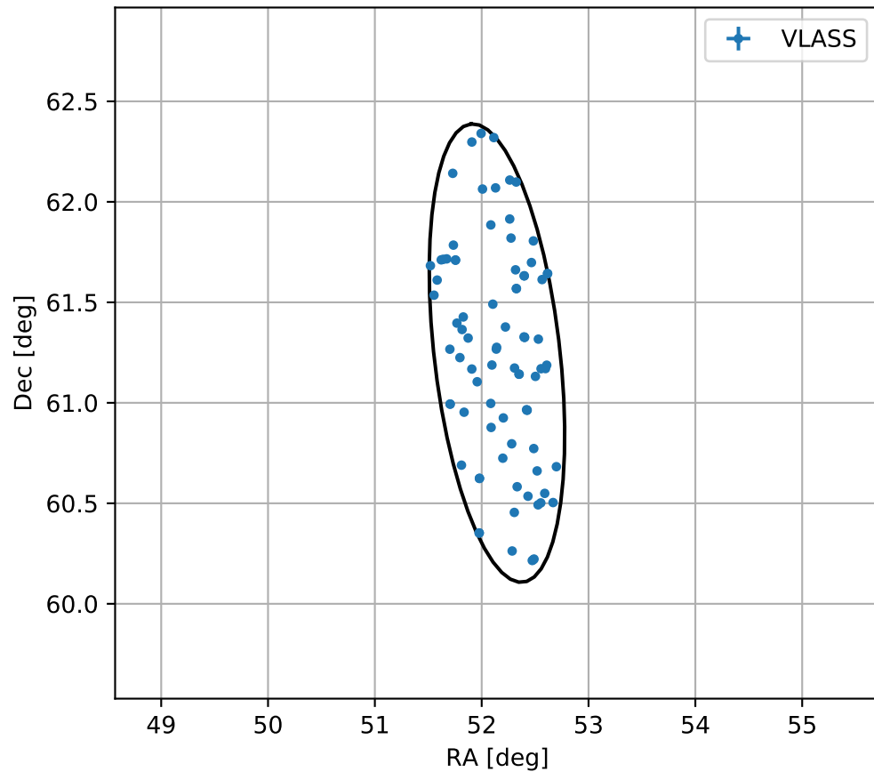
4FGL J0328.5+6114
