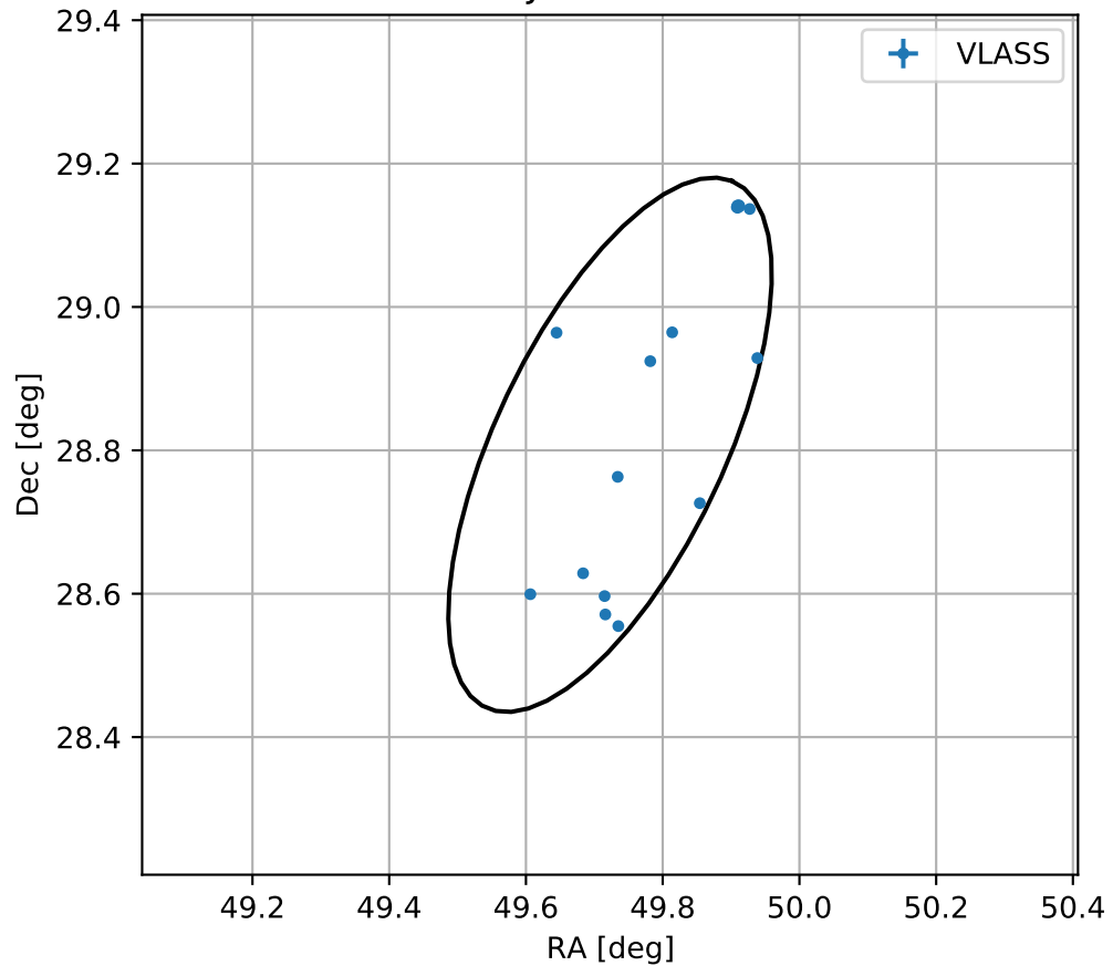
4FGL J0318.8+2848
