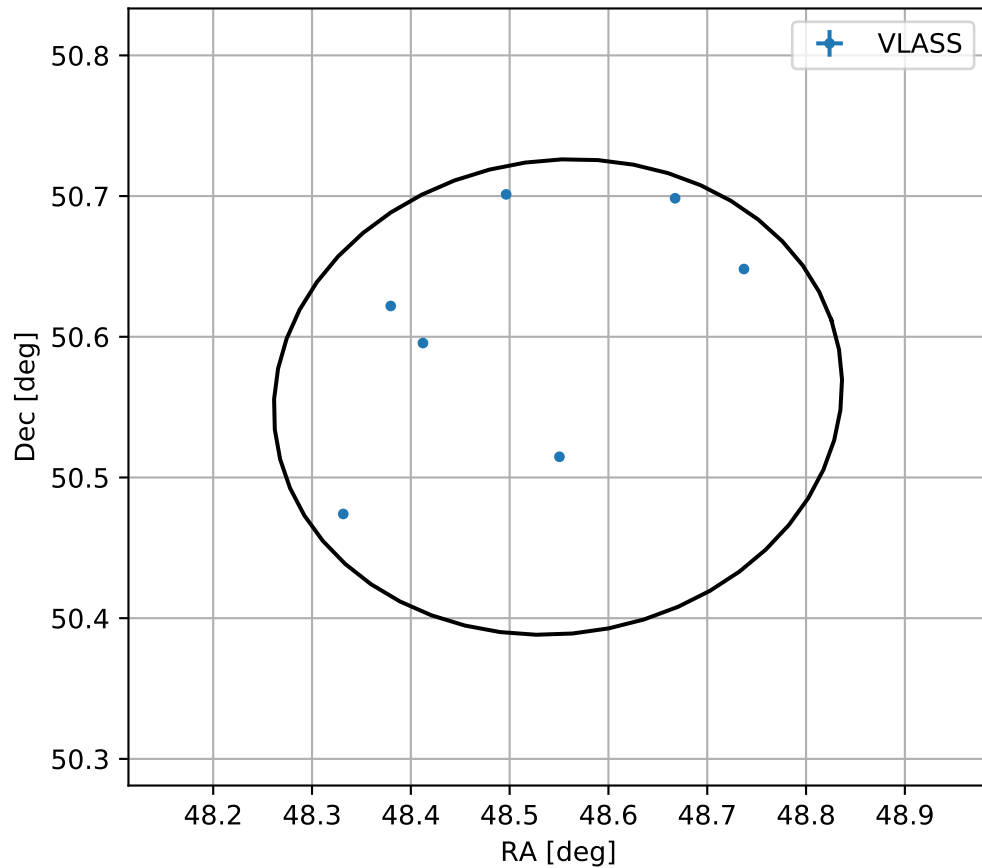
4FGL J0314.1+5033
