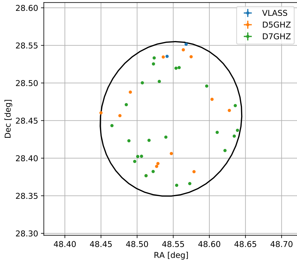
4FGL J0314.1+2827
