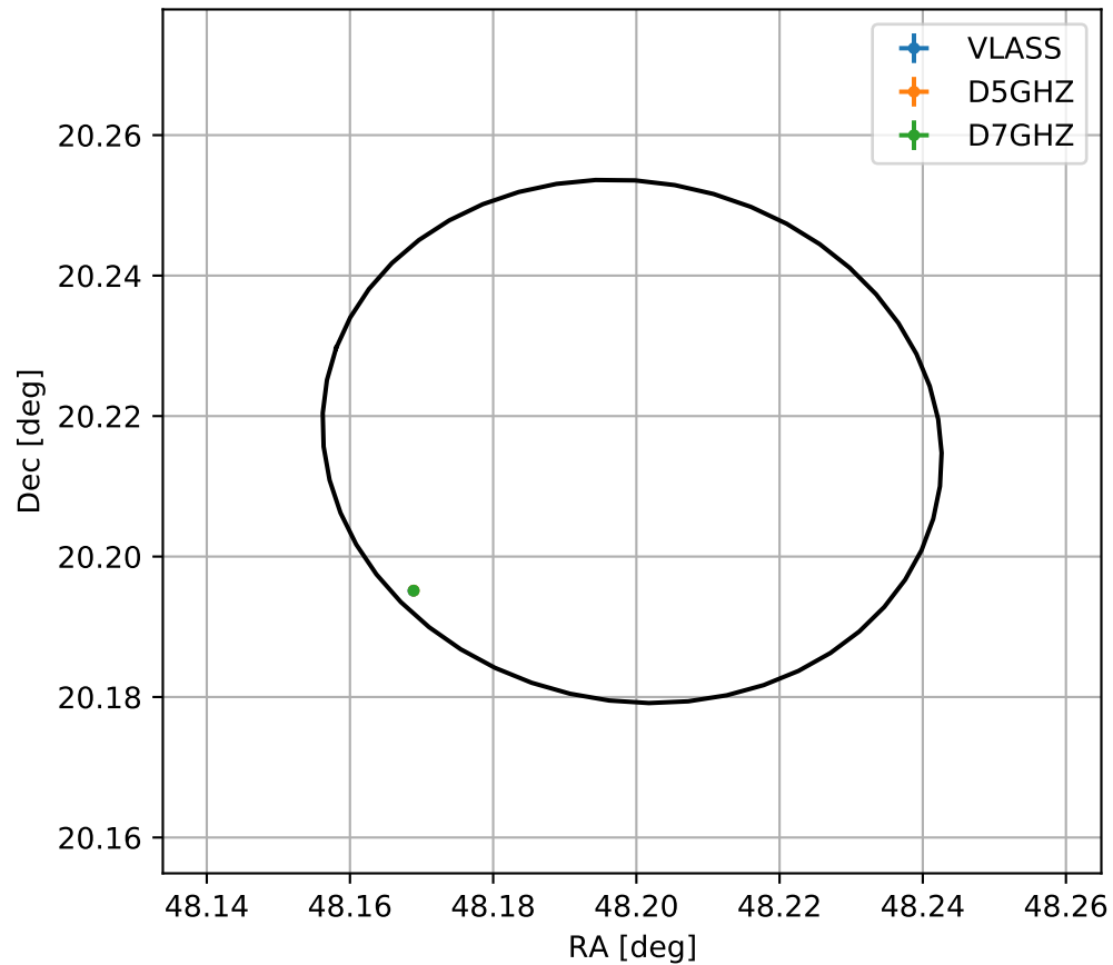
4FGL J0312.7+2012
