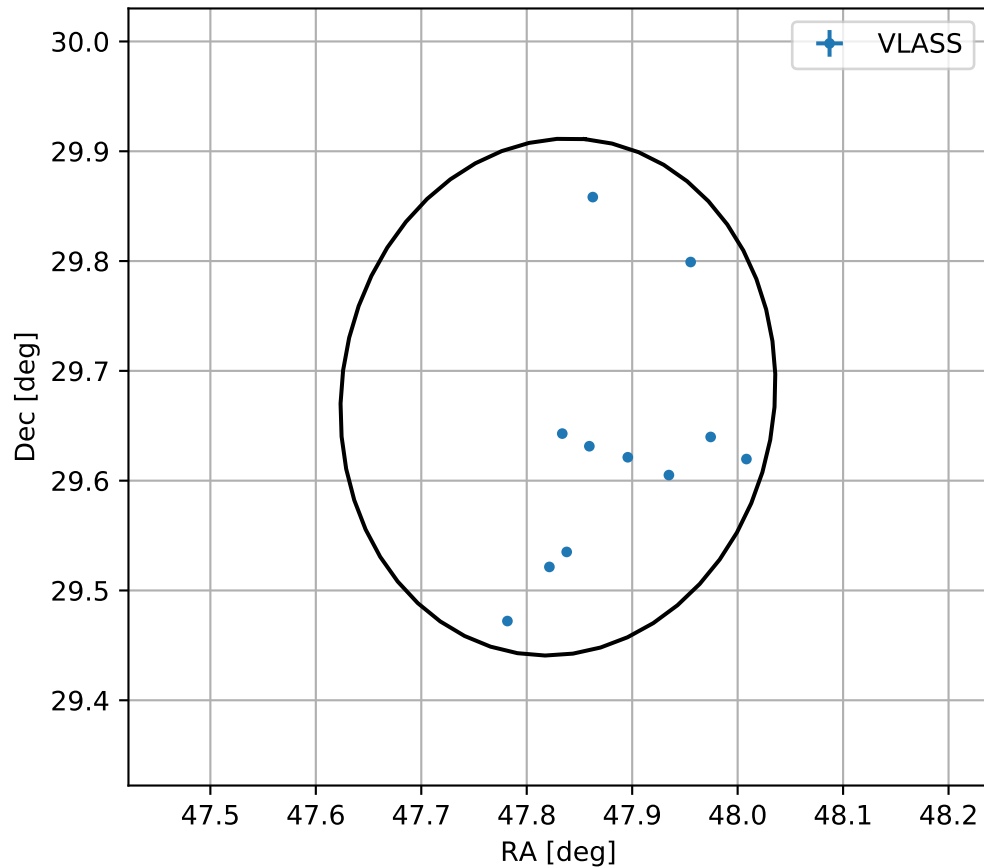
4FGL J0311.3+2940
