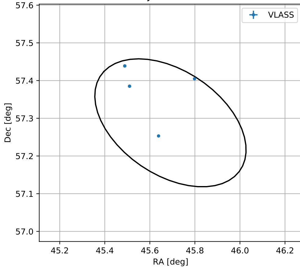
4FGL J0302.7+5717
