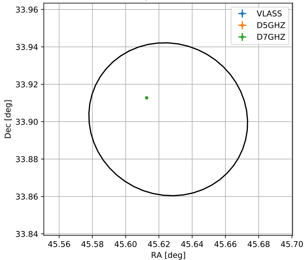
4FGL J0302.5+3354
