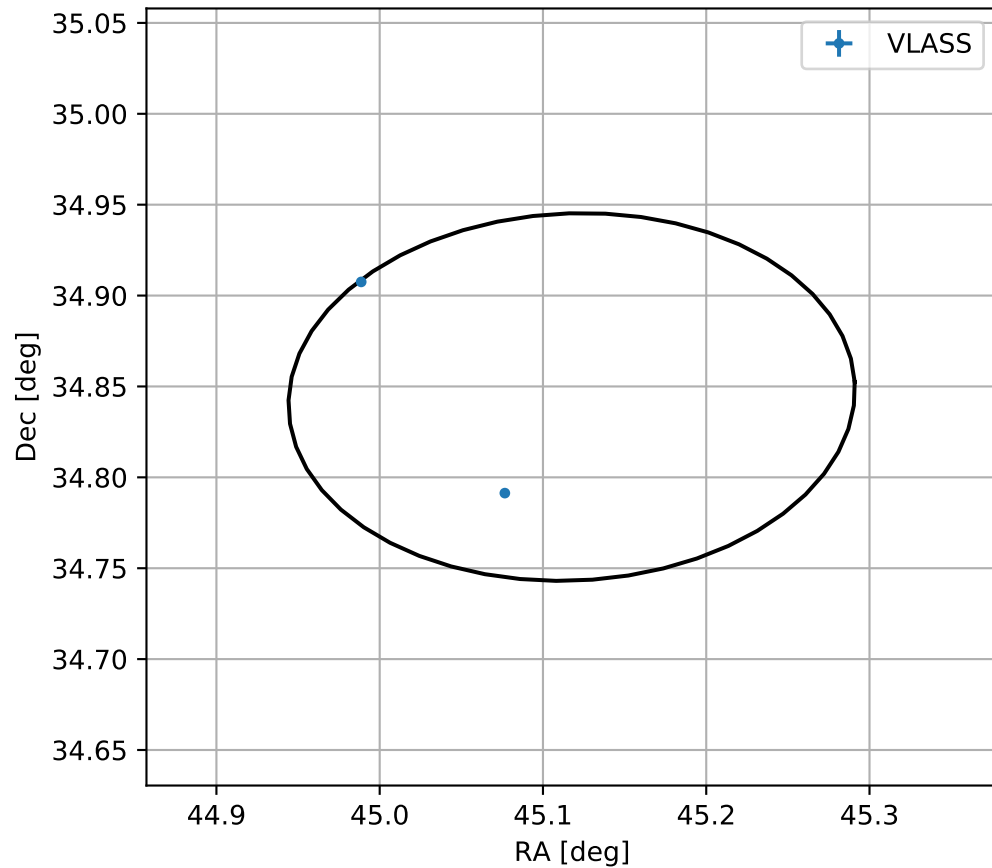
4FGL J0300.4+3450
