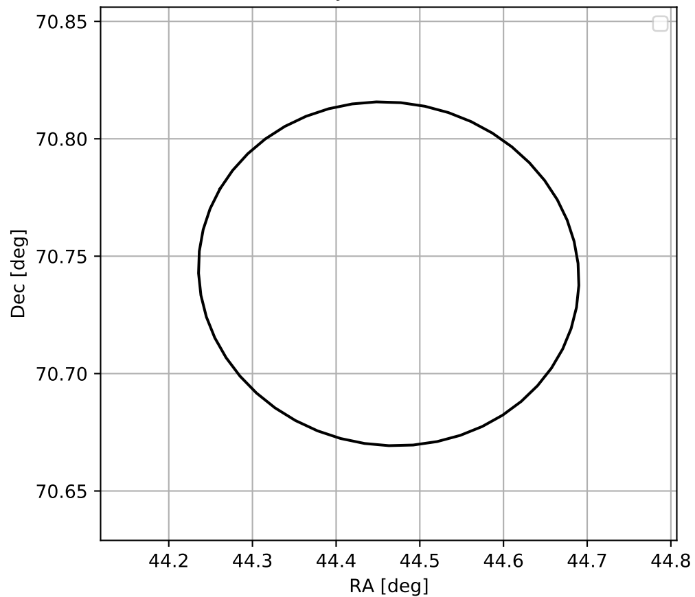
4FGL J0257.8+7044
