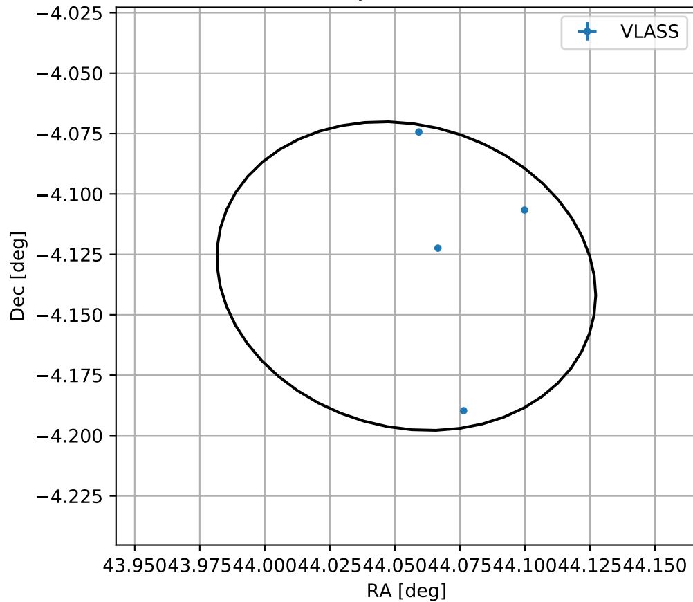
4FGL J0256.2-0408
